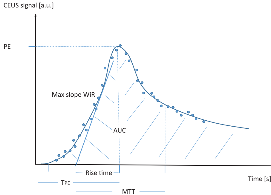
Fig. 1. CEUS standard time–intensity curve after UCA bolus injection. Blue dots represent real, linearized values; a fitting curve provides the following CEUS parameters: PE (in a.u.), the maximum signal intensity of the enhancement curve; T_{PE} (s), duration from UCA application to maximum signal; WiR (a.u./s), the maximum slope to peak; RT (s), that is, T_{PE} – time where the maximum slope line originates; AUC (a.u. \times s), area under the TIC curve; MTT (s), fitting model dependent. a.u. = arbitrary units; AUC = area under the curve; CEUS = contrast-enhanced ultrasound; MTT = mean transit time; PE = peak enhancement; RT = rise time; T_{PE} = time to peak; UCA = ultrasound contrast agent; WiR = wash-in rate.
