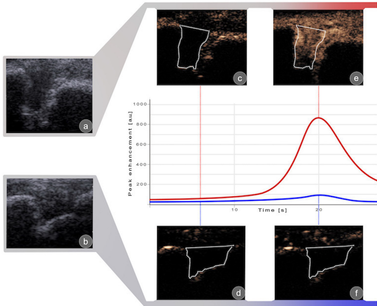
Fig. 4. Time–intensity curves of infected (red) and aseptic (blue) tibial non-unions before revision surgery. (a, c, e) Corresponding ultrasound images with the non-union gap in B-mode (a) and in contrast mode before (c) and after (e) contrast agent inflow in case of infection. (b, d, f) Corresponding ultrasound images with the non-union gap in B-mode (b) and in contrast mode before (d) and after (f) contrast agent inflow in the case of an aseptic non-union. Informed patient consent for publication available. a.u. = arbitrary units.
